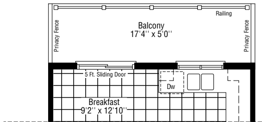
Part Main Floor Plan With Full Length Balcony (For Blocks 17-20 Only)
