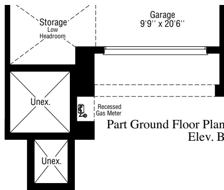
Part Basement Floor Plan Elev. B
