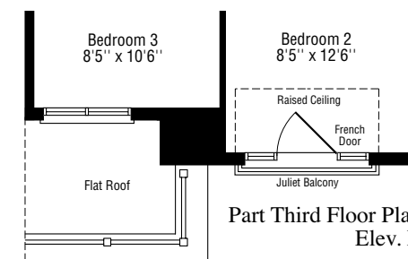
Third Floor Plan Elev. A
