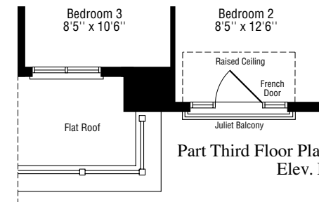
Third Floor Plan Elev. A
