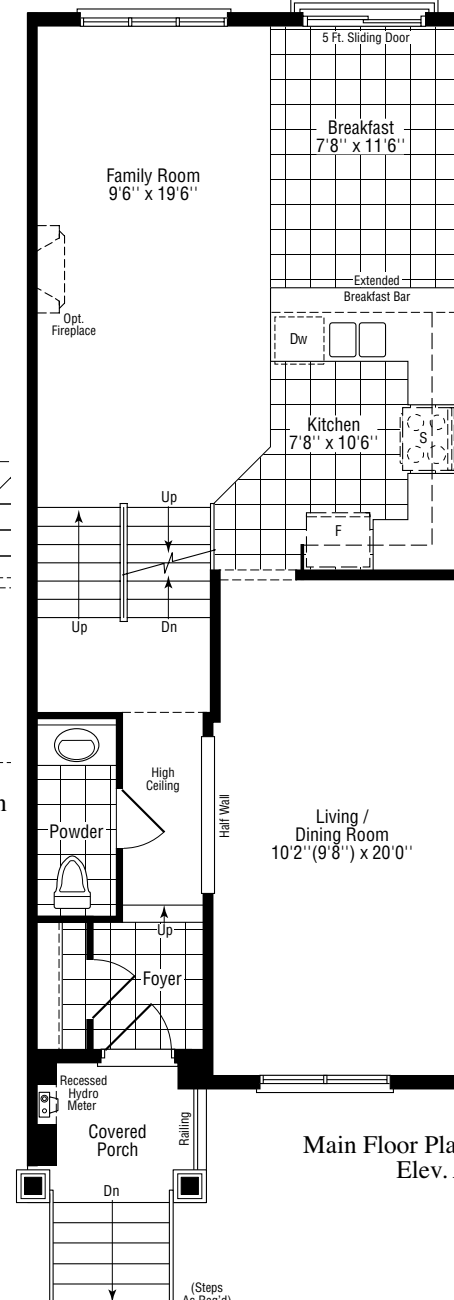
Part Main Floor Plan With Full Length Balcony (For Blocks 17-20 Only)
